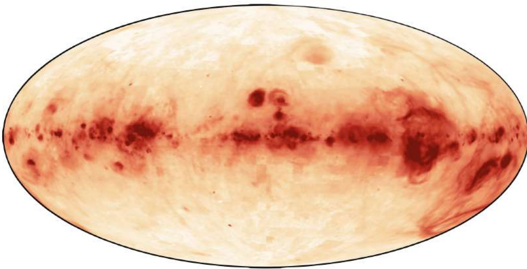
FIGURE 10.29 – Emission H\alpha Galactique [65].
