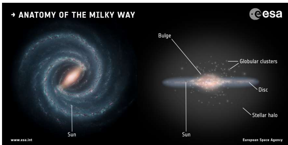
FIGURE 12.2 – Structure de la Galaxie
