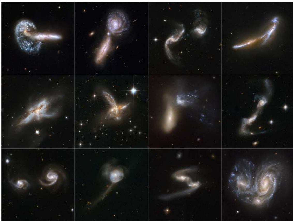
FIGURE 13.18 – Galaxies en interaction. [NASA, ESA, the Hubble Heritage (STScI/AURA)-ESA/Hubble Collaboration, and A. Evans (University of Virginia, Charlottesville/NRAO/Stony Brook University)].
