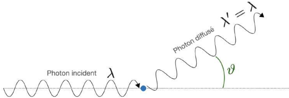
FIGURE 2.12 – Diffusion Thomson.
