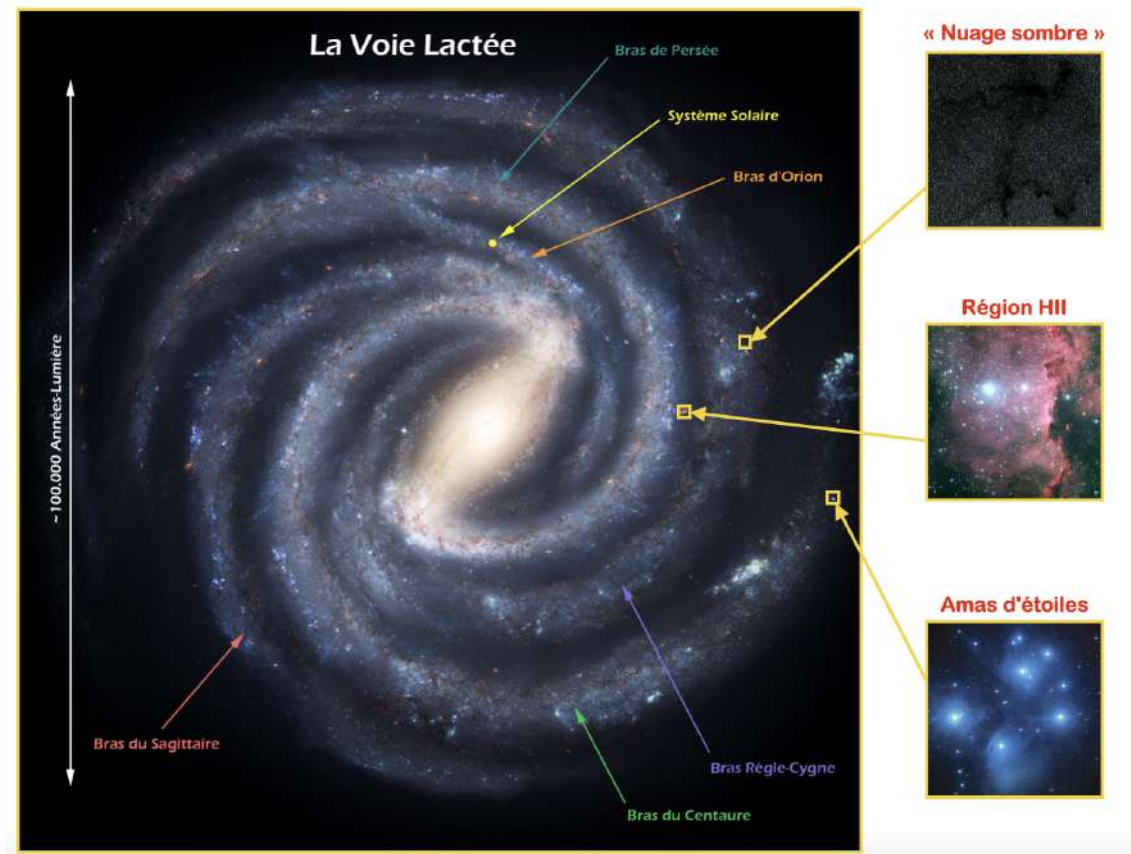
FIGURE 10.8 – Structure de la Galaxie
